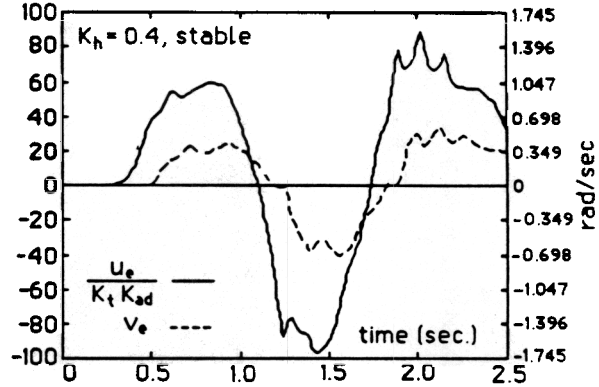
Figure 8: Stable, ( K_h = 0.4 )
